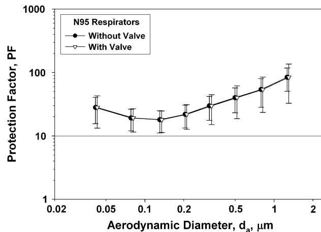
Fig. 3. The comparison of PFs against particles in bacterial and viral size ranges between respirators without (N95 Respirator C) and with (N95 Respirator D) exhalation valves. The tests were performed when the N95 respirators were donned on human subjects. Each data point represents an average and standard deviation of 36 observations for N95 Respirator C and 9 observations for N95 Respirator D.
